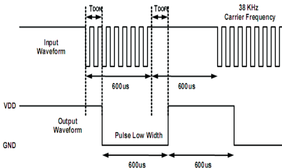
Figure 1. Input burst wave form
