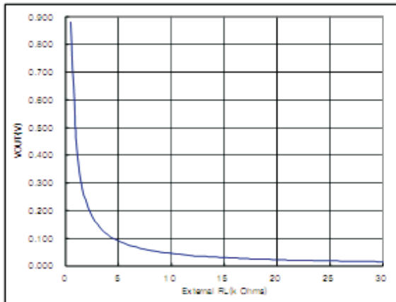
Figure 4. V_{OL} vs Pull-up resistance
