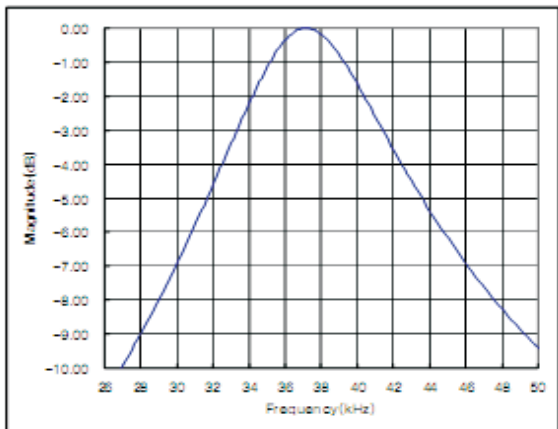
Figure 2. Typical Band-pass Curve
