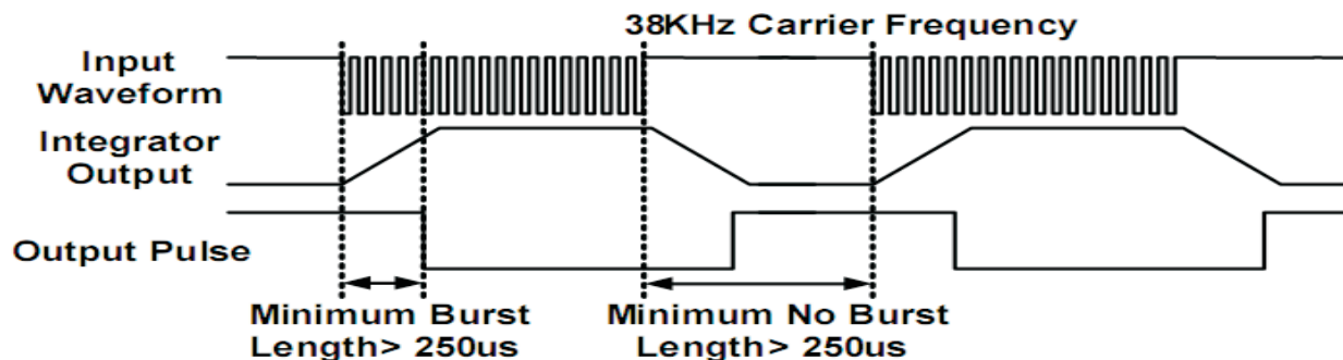
Figure 10. Minimum burst length & No burst length
