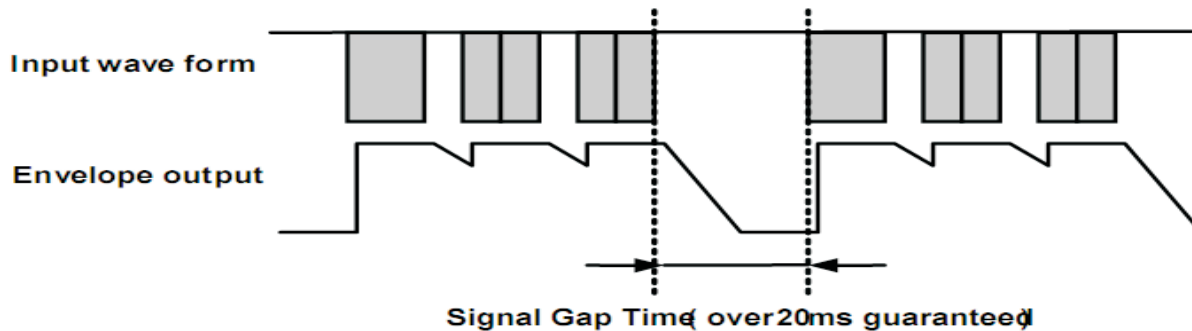
Figure 11. Recommended repeated code format
