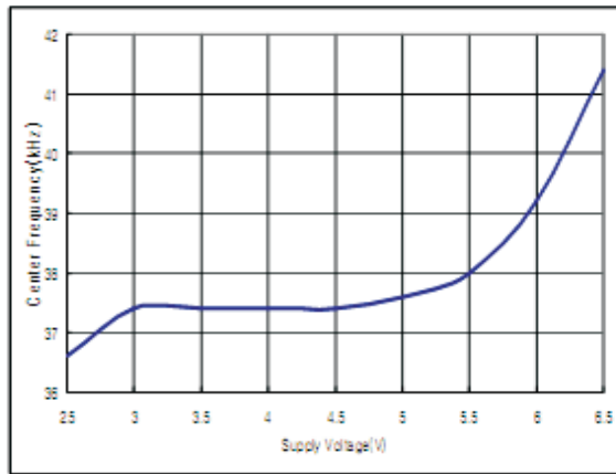
Figure 3. Center Frequency vs supply voltage
